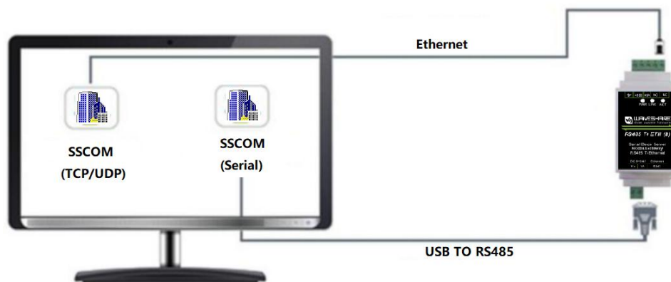
Figure 9 Schematic diagram of TCP communication
